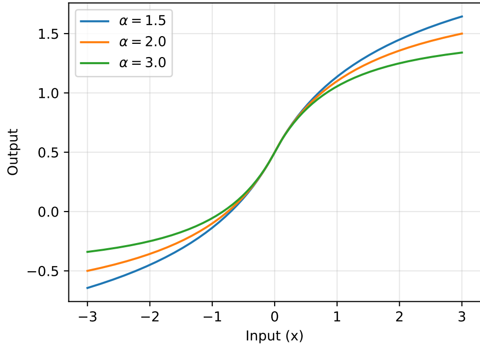
q-PseudoSpike Original Function
