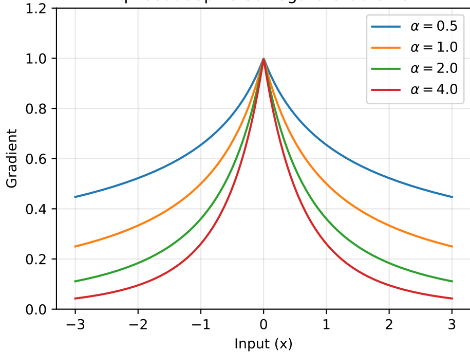
q-PseudoSpike Surrogate Gradients
