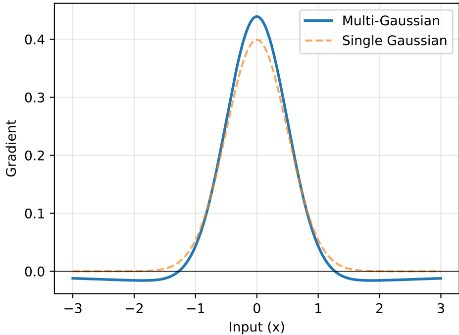
Multi-Gaussian vs Single Gaussian
