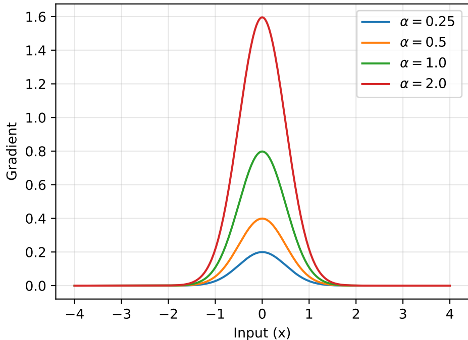
Scaling Effect ( \sigma=0.5 )
