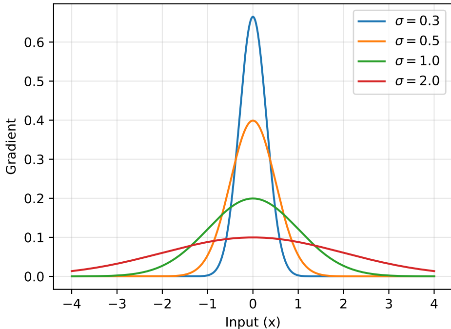
Gaussian Gradients ( \alpha=0.5 )
