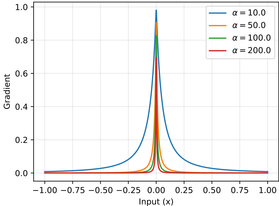
Inverse-Square Gradients
