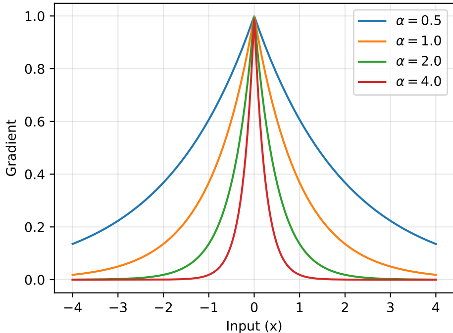
SLAYER Surrogate Gradients
