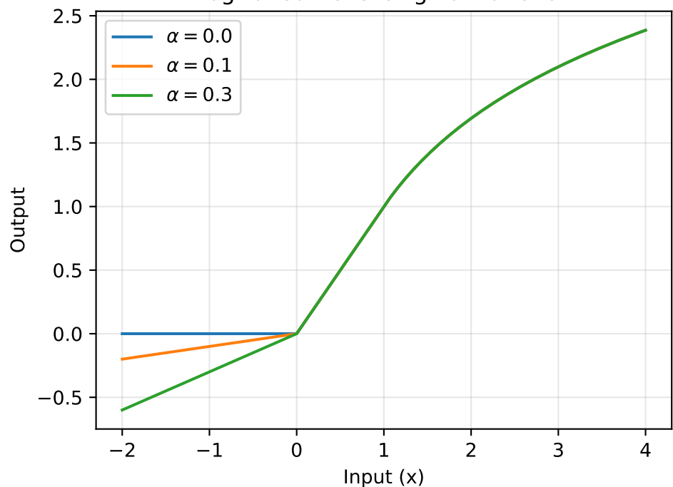
Log-tailed ReLU Original Function
