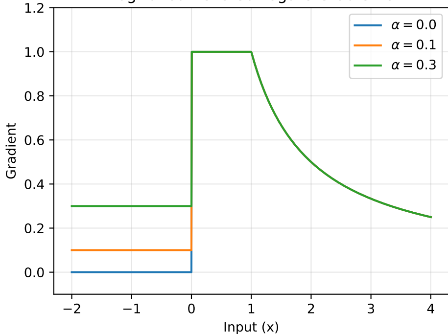
Log-tailed ReLU Surrogate Gradients
