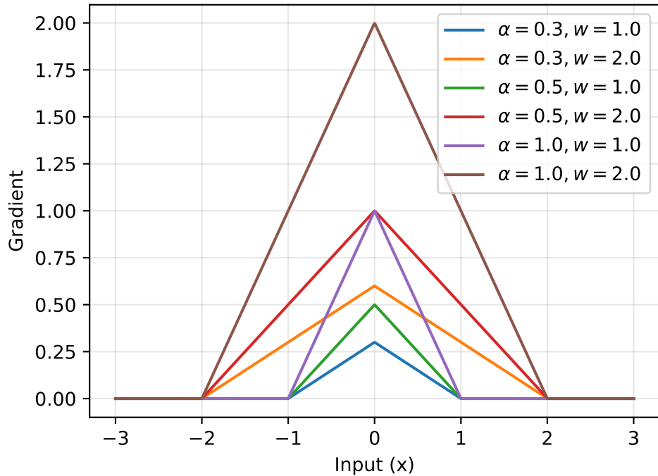
ReLU Surrogate Gradients
