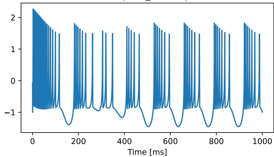
irregular_bursting
