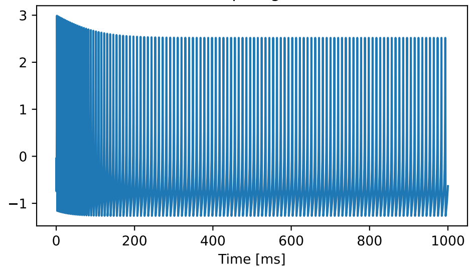
irregular_spiking
