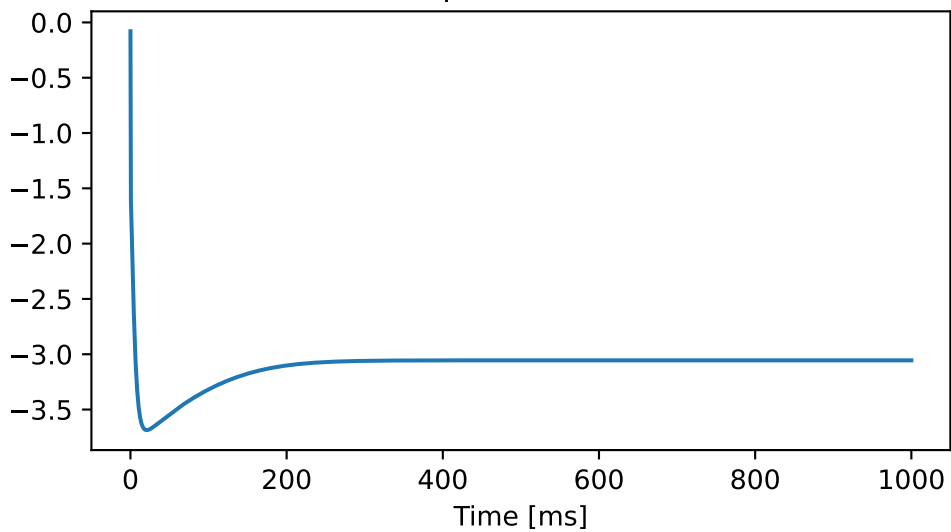
bursting
