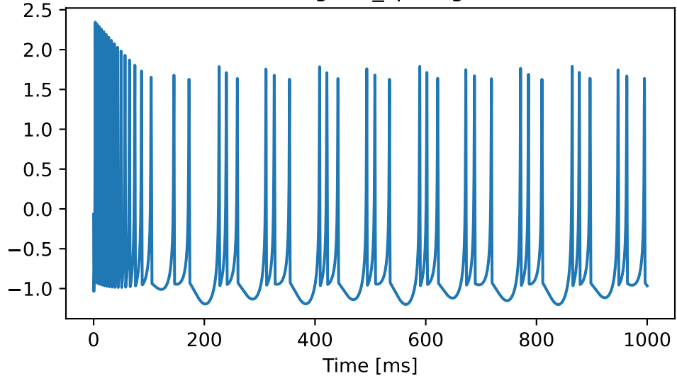
irregular_spiking
